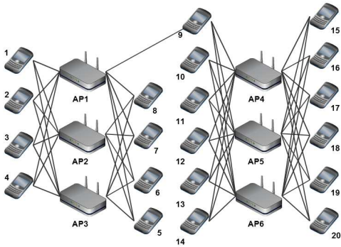
Figure 2: Illustrating non-localizability
